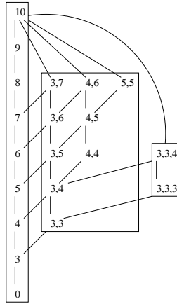
Figure 6-1: \Pi_{10,3} , in three leveled subposets.
