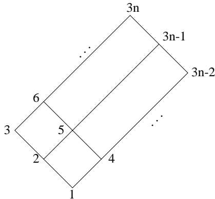
Figure 4-3: A natural labeling of \mathbf{3} \times \mathbf{n} .
