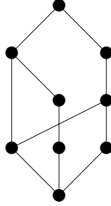
Figure 1-4: An unranked but leveled poset.
