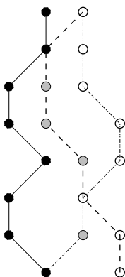
Figure 2-2: Salvaging a dead end.
