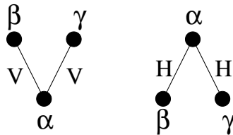
Figure 2-4: Two special cases.
